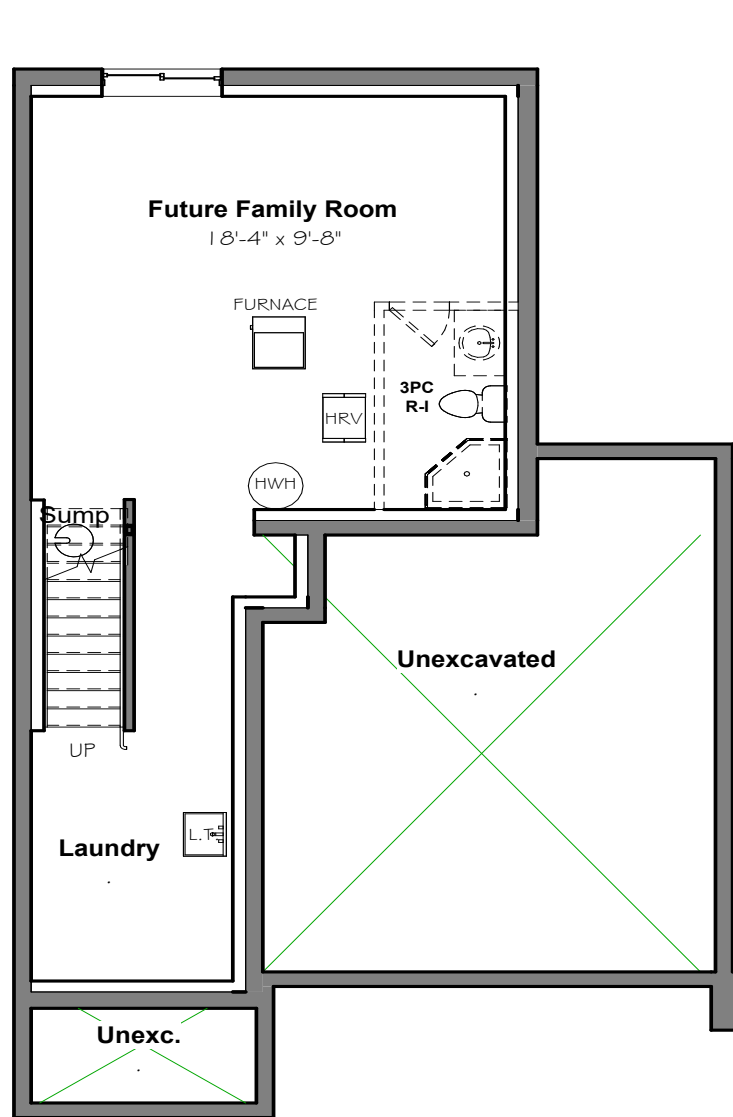
BASEMENT
